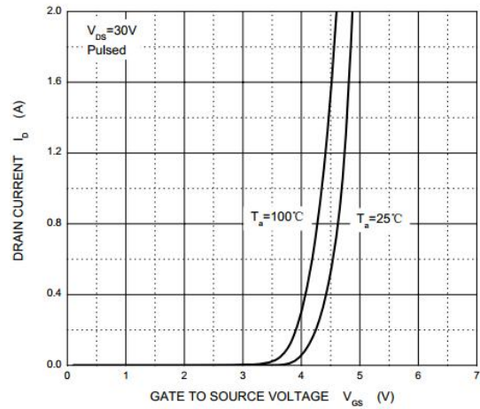
Transfer Characterisics
