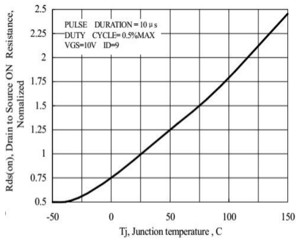
Rdson-Junction Temperature
