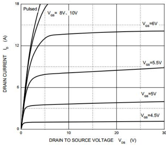
Output Characterisics
