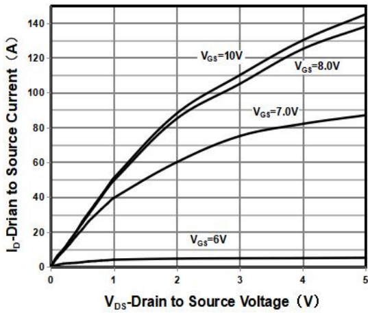
Output Characterisics
