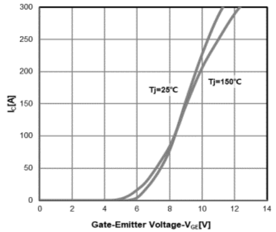
Transfer Characteristics ( V_{CE} = 15V )
