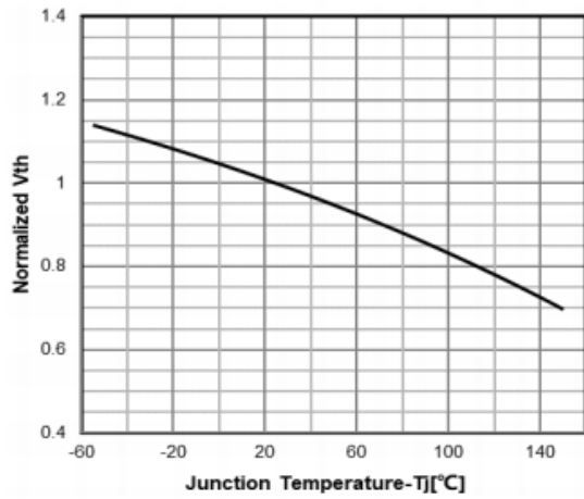
Normalized V_{GE(th)} vs. temperature
