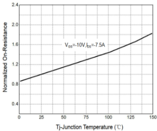
Rdson-JunctionTemperature
