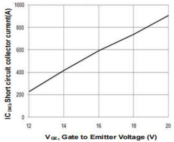
Typ. short circuit collector current as a function of gate-emitter voltage ( V_{ce} \leq 400\text{V} , T_j \leq 150^\circ\text{C} )
