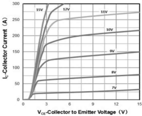
Output Characterisics
