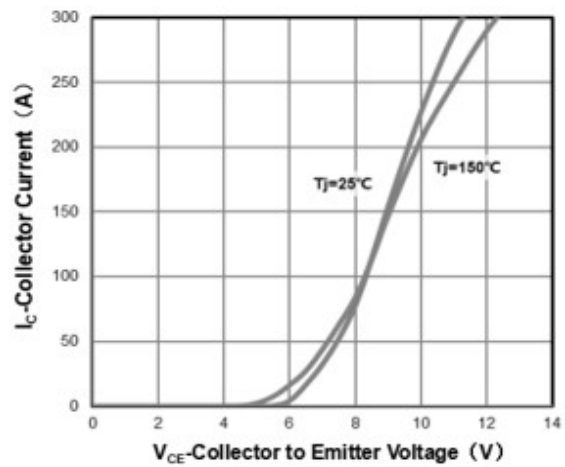
Transfer Characterisics
