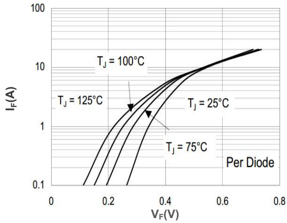
Forward Characteristics Per Diode
