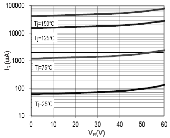
Reverse Characteristics Per Diode
